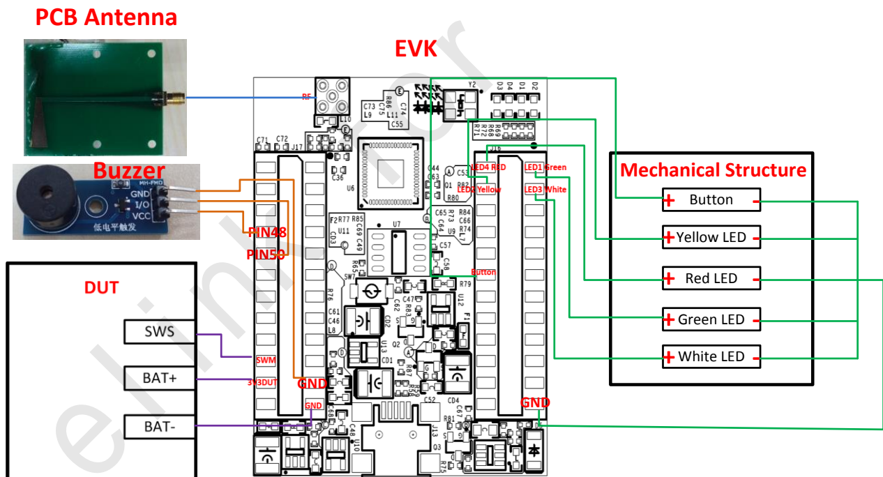
Figure 8 Cable connection chart
