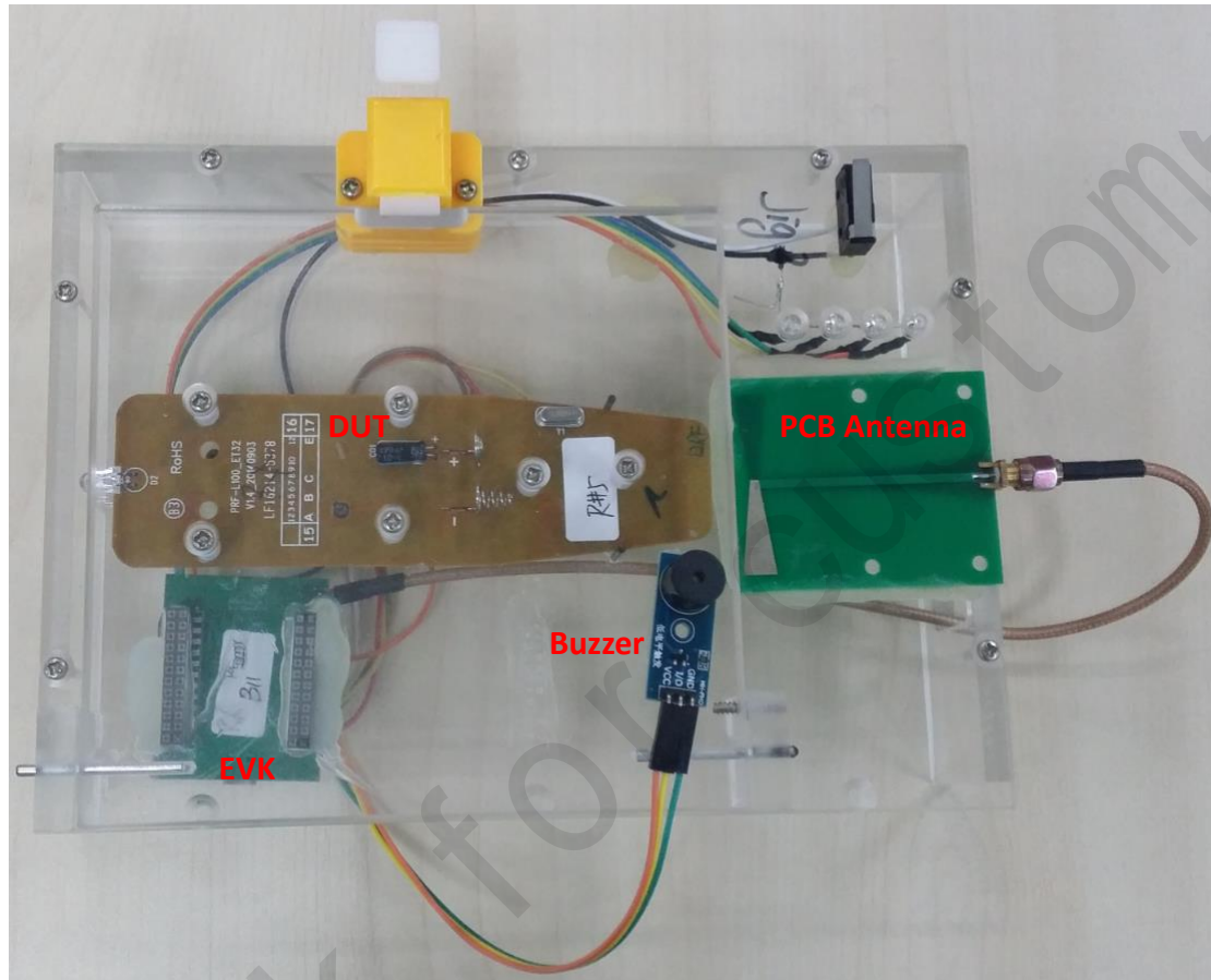
Figure 9 BLE 1x1 Test System 2.1
