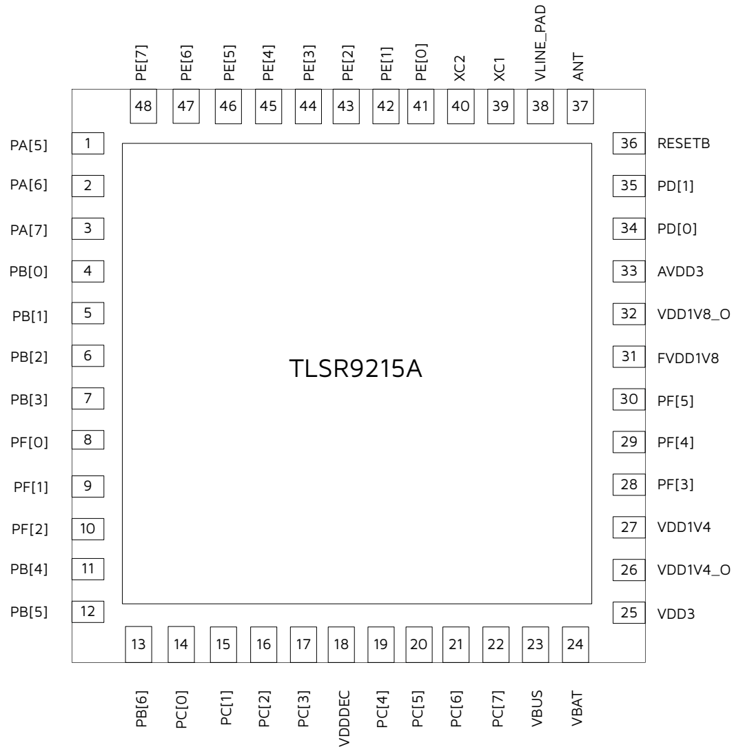
Figure 1-4 Pin Assignment for TLSR9215A
