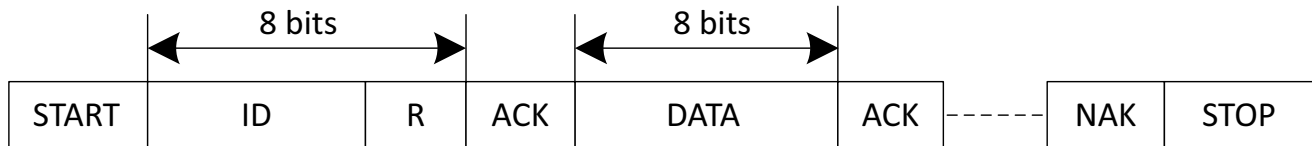
Figure 9-6 Write Format in Slave Mode
