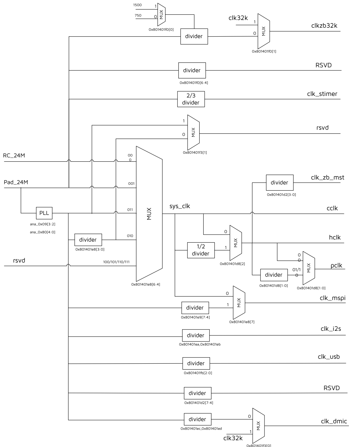
Figure 6-1 Clock Source
