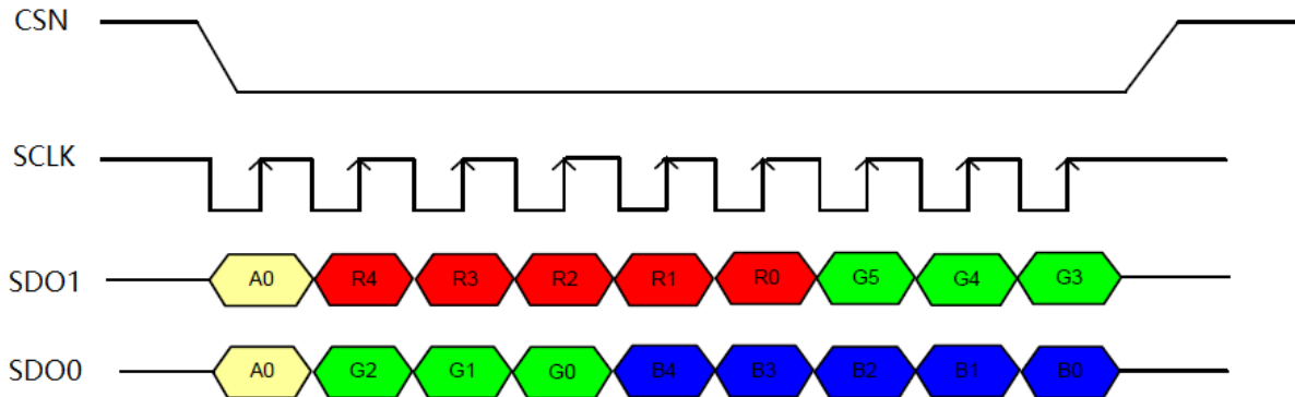
Figure 9-17 RGB666 Pixel Transition
