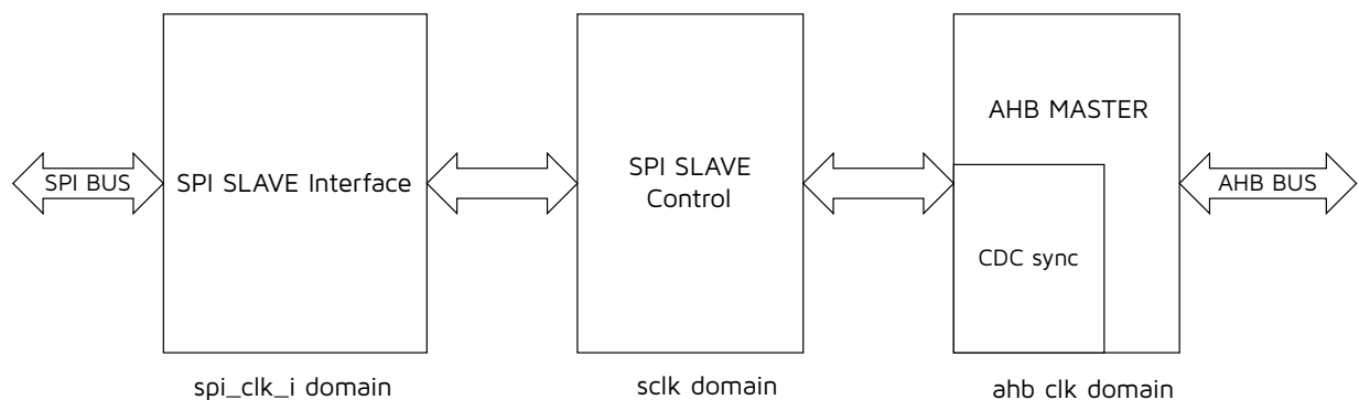
Figure 9-22 SPI_SLV Diagram
