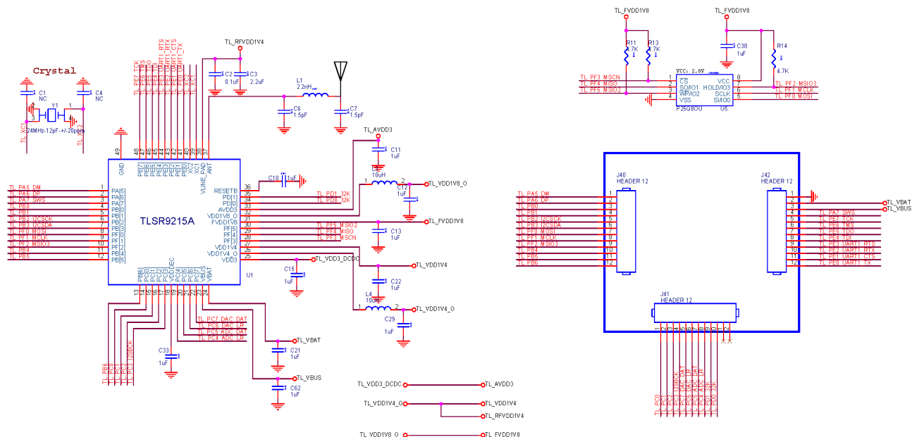
Figure 3-1 Schematic of TLSR9215
