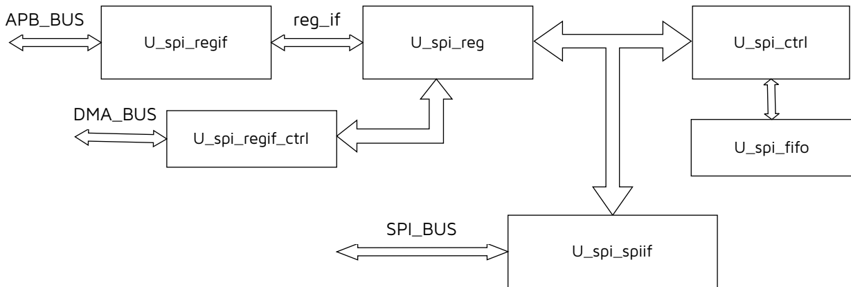
Figure 9-19 PSPI Diagram
