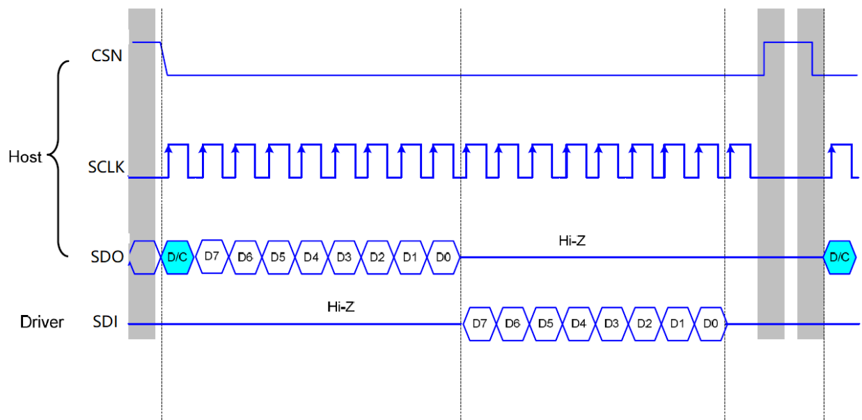
Figure 9-12 3-Line Read Sequence
