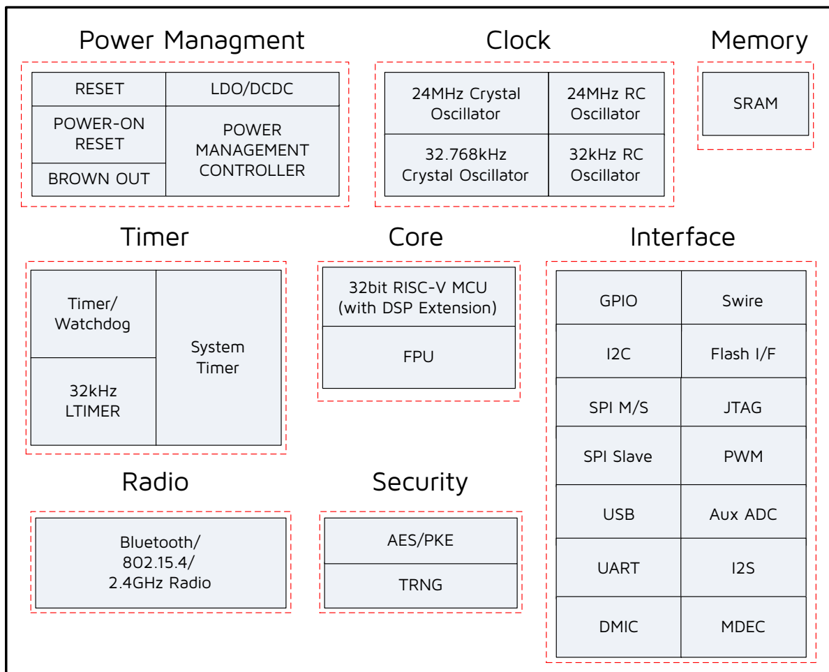
Figure 1-1 Block Diagram of the System
