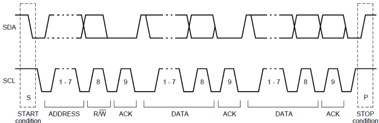
Figure 9-3 I2C Timing
