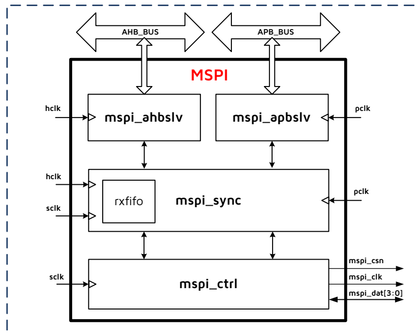
Figure 9-7 Memory SPI Diagram
