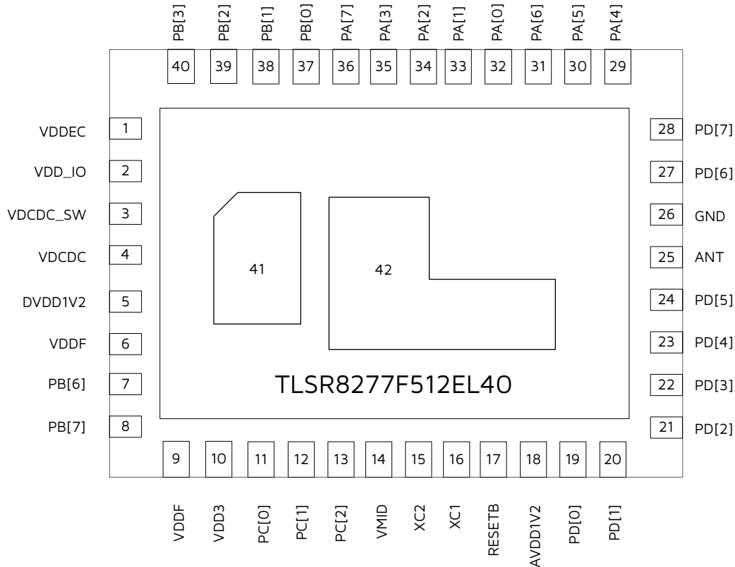
Figure 1-3 Pin Assignments for TLSR8277F512EL40
