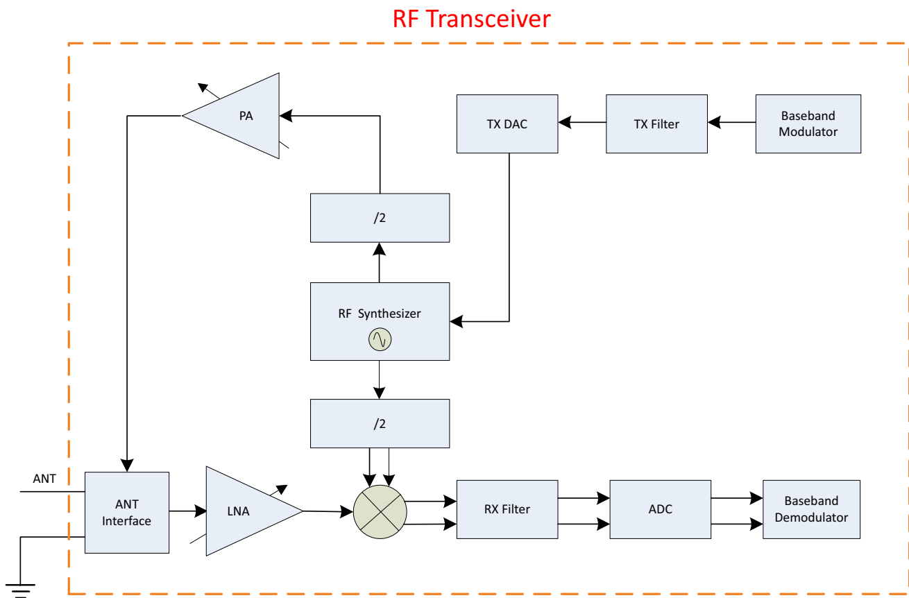
Figure 3-1 Block Diagram of RF Transceiver
