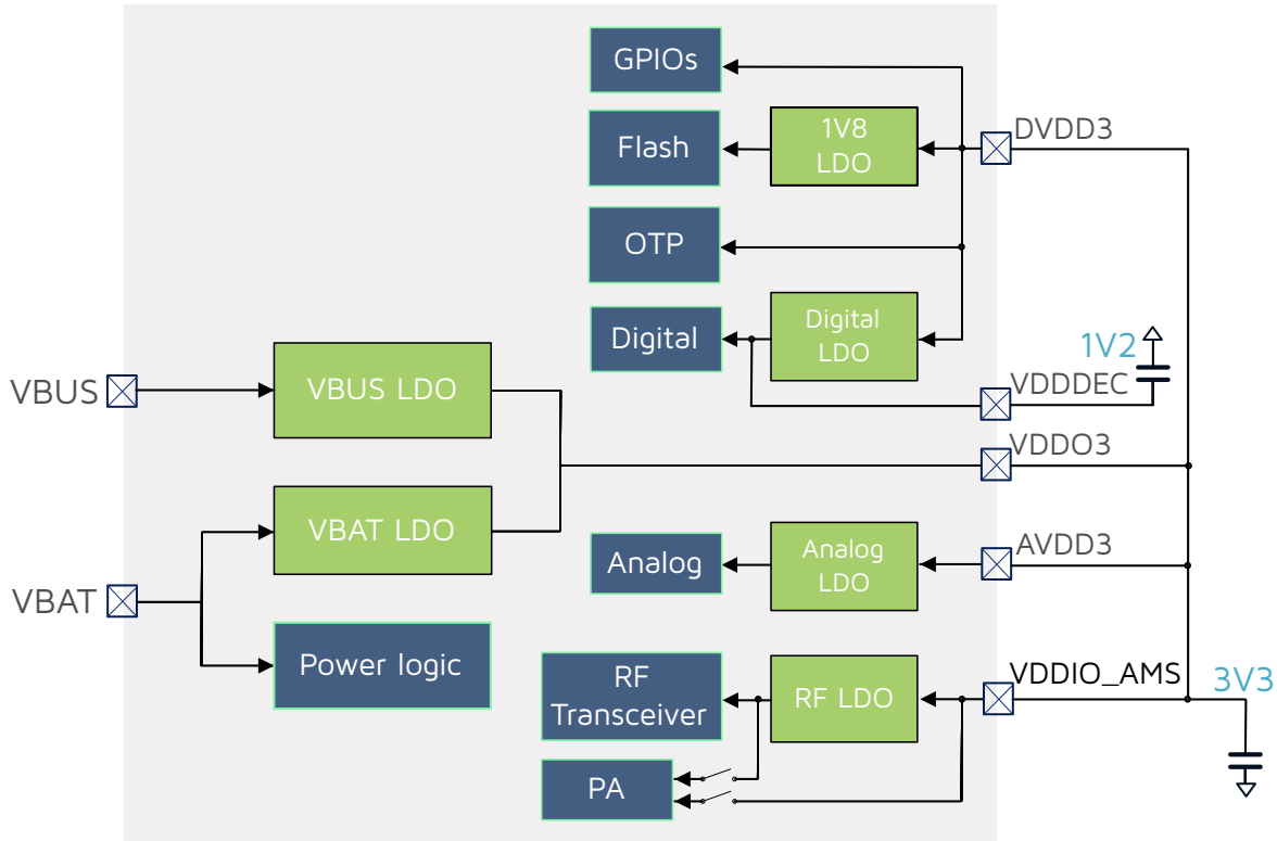
Figure 2-7 LDO
