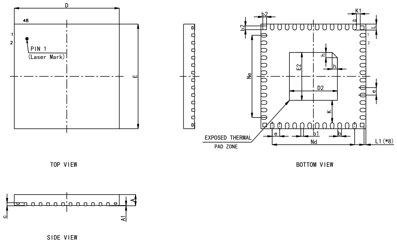
Figure 1-2 Package of TLSR8278F1KET48 (H)
