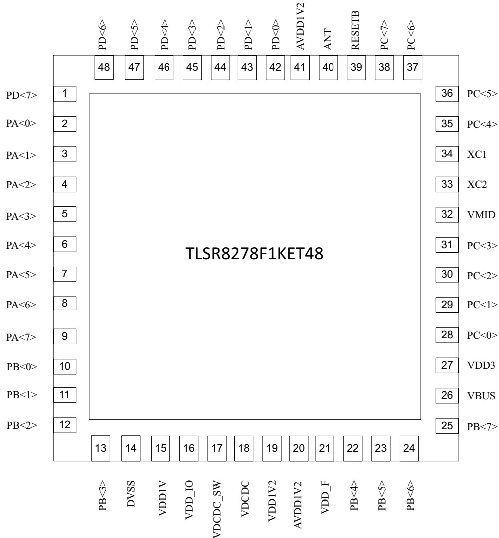
Figure 1-5 Pin Assignments for TLSR8278F1KET48
