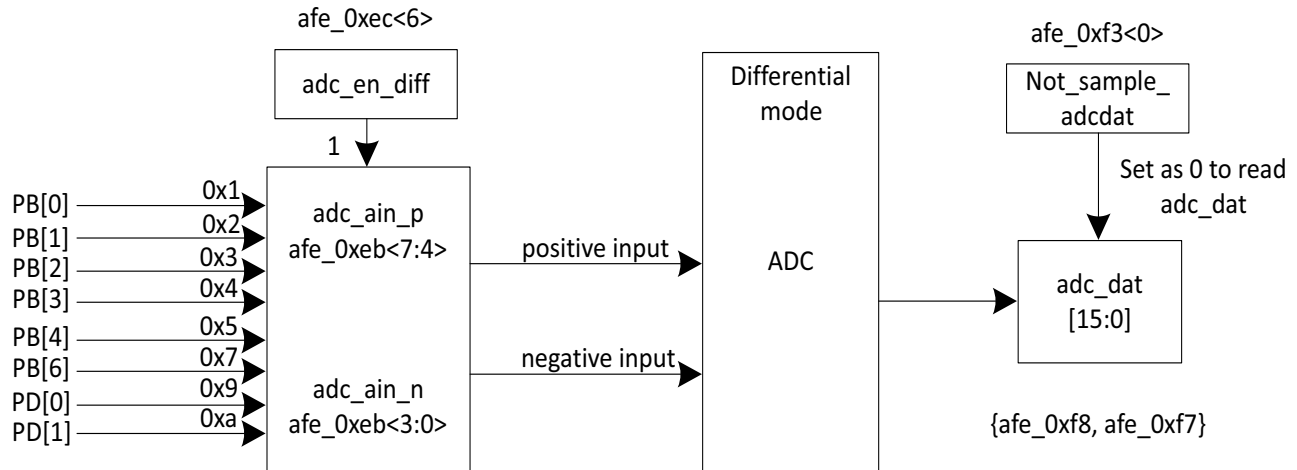
Figure 13-1 ADC Diagram For TLSR9517
