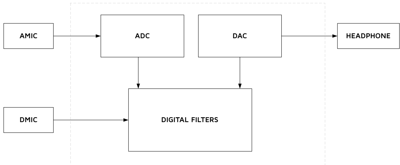
Figure 5-1 Audio CODEC
