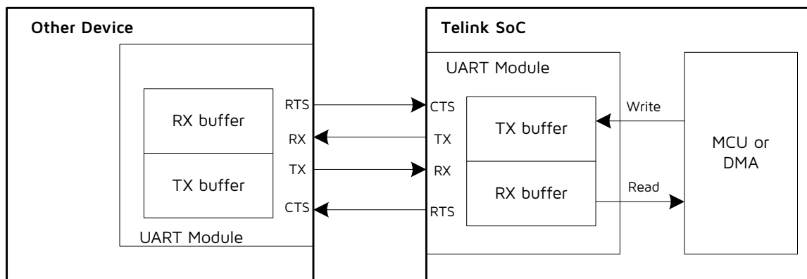
Figure 10-22 UART Communication
