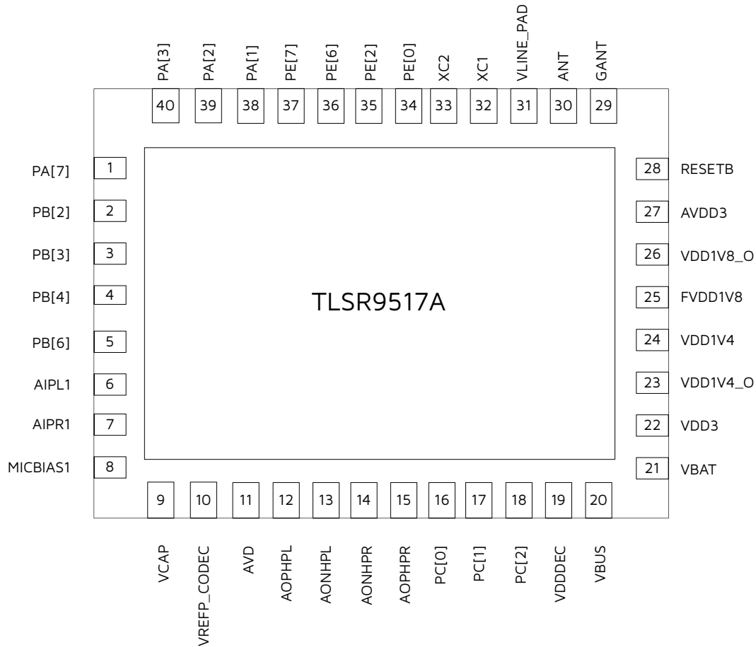
Figure 1-4 Pin Assignment for TLSR9517A
