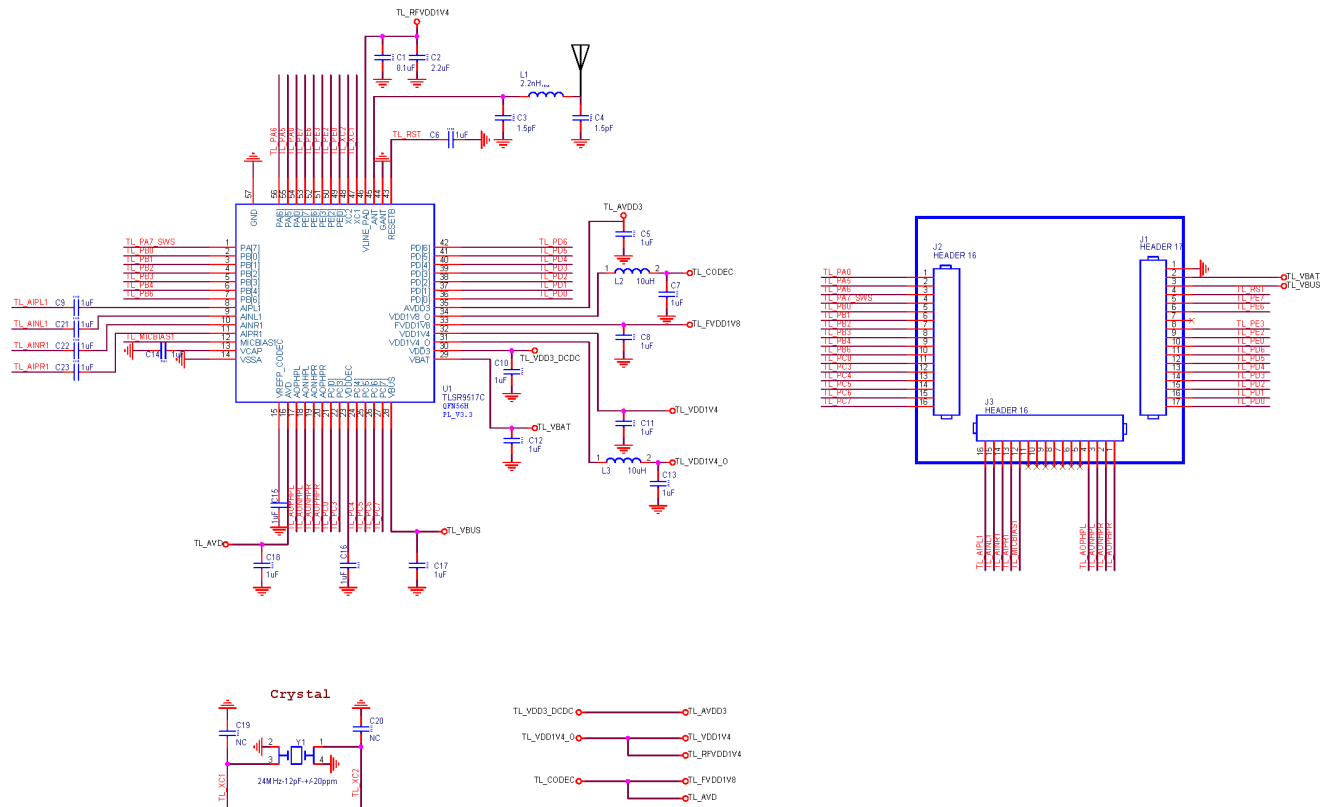
Figure 3-3 Schematic of TLSR9517C
