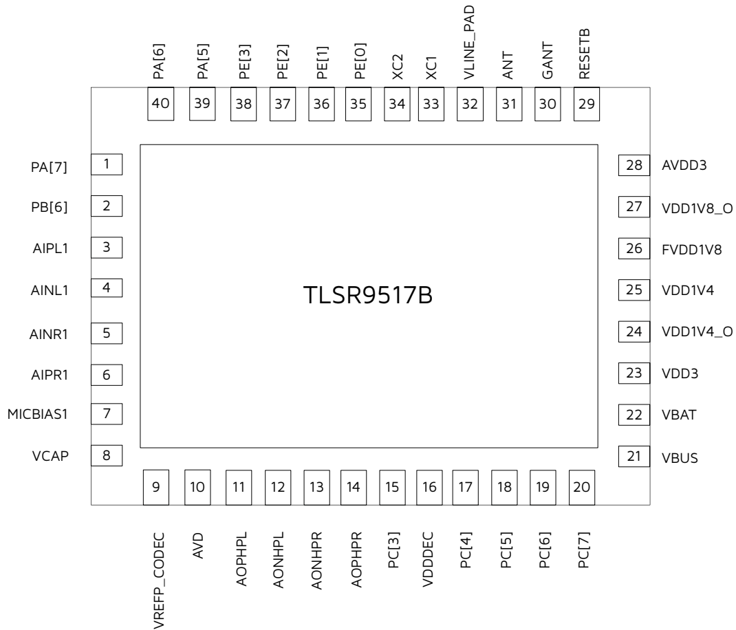
Figure 1-5 Pin Assignment of TLSR9517B
