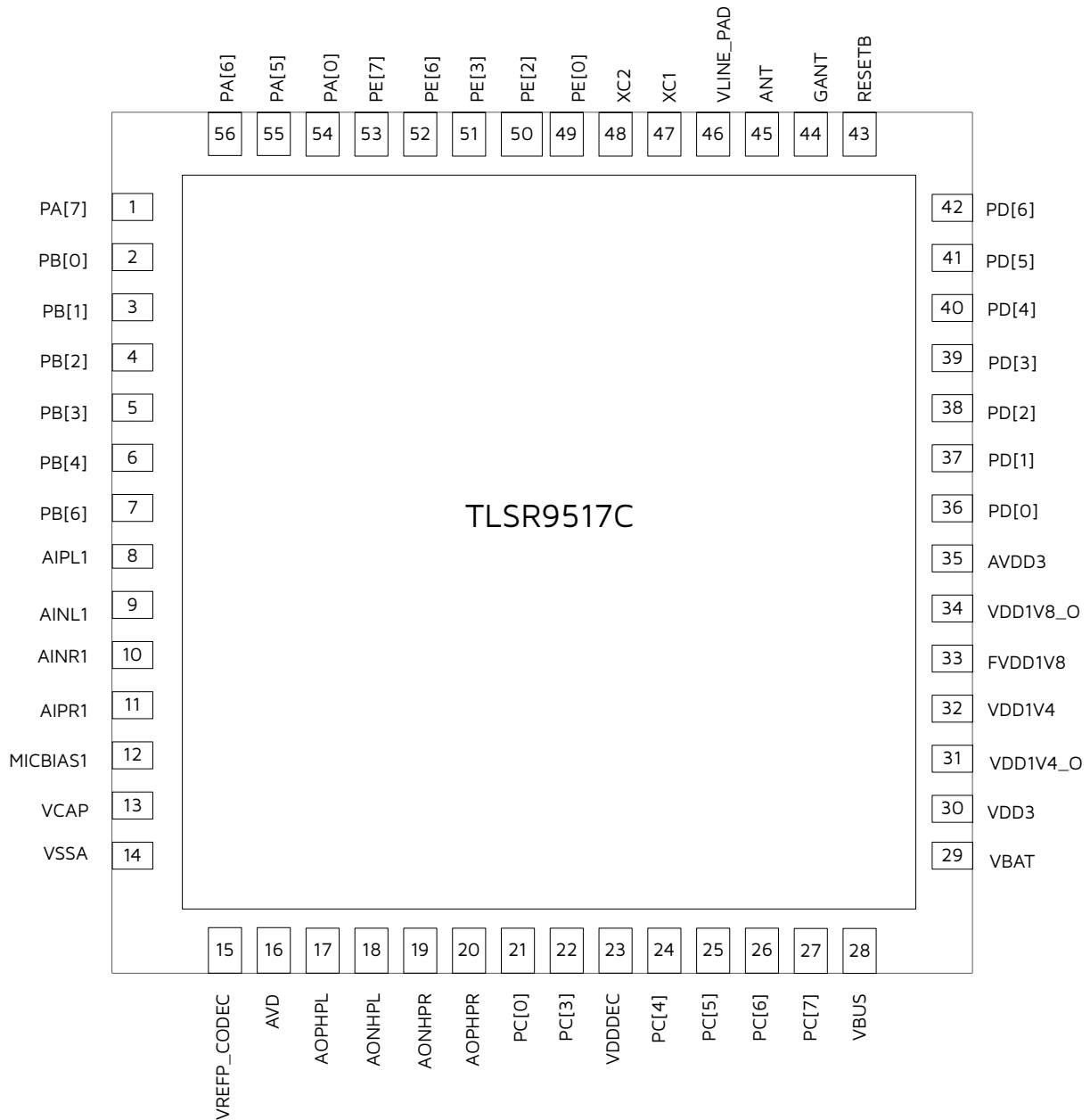
Figure 1-6 Pin Assignment of TLSR9517C
