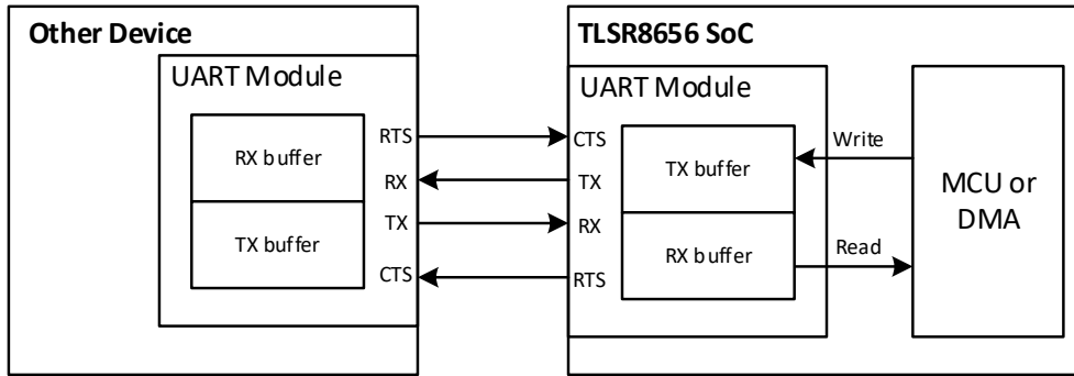
Figure 7- 10 UART communication
