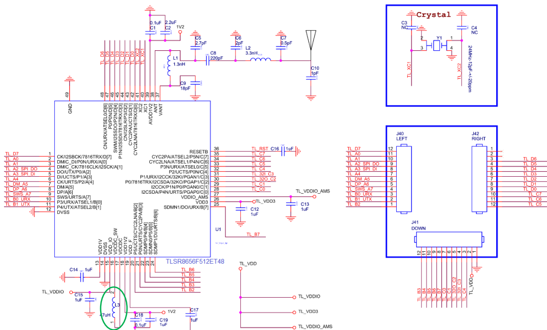
Figure 16- 2 Schematic for TLR8656F512ET48
