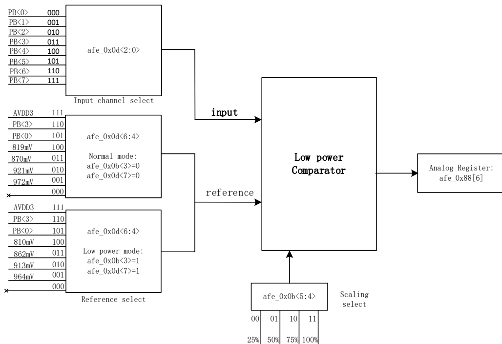
Figure 13- 1 Block diagram of low power comparator
