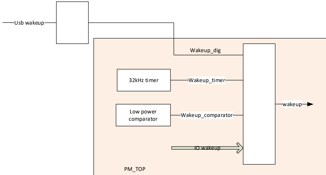
Figure 2- 6 Wakeup sources
