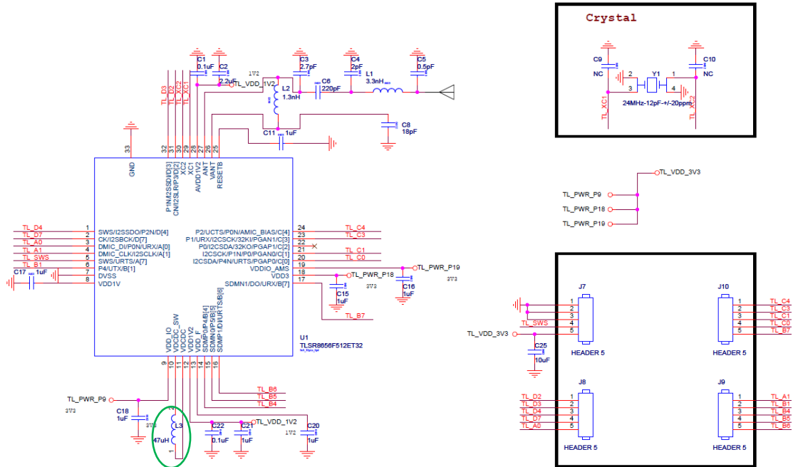
Figure 16- 1 Schematic for TLSR8656F512ET32
