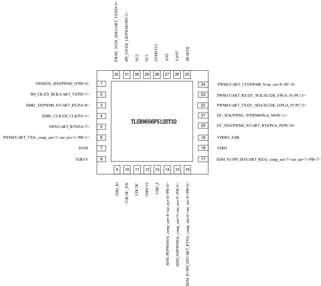
Figure 1- 4 Pin assignment for TSLR8656F512ET32
