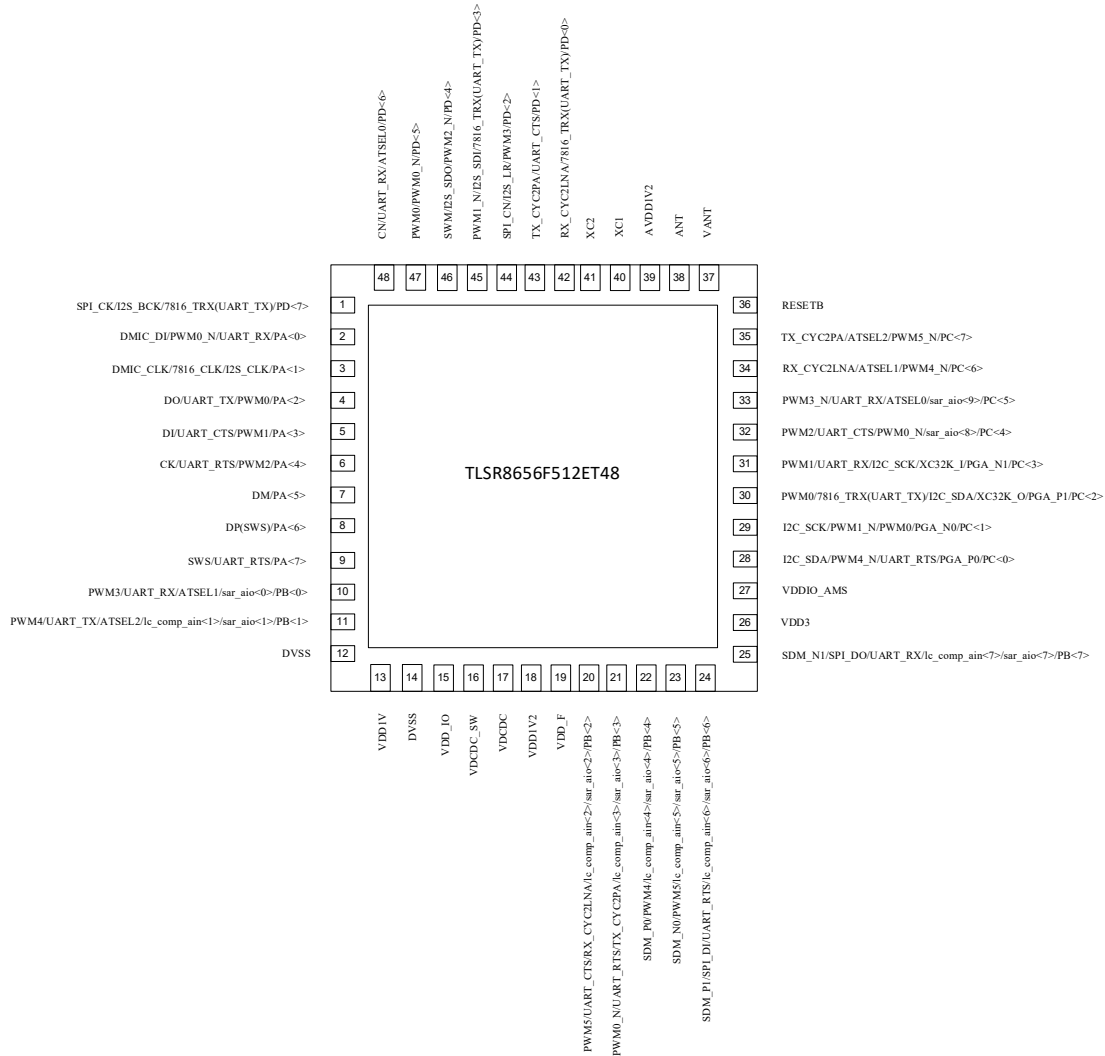
Figure 1- 5 Pin assignment for TLSR8656F512ET48
