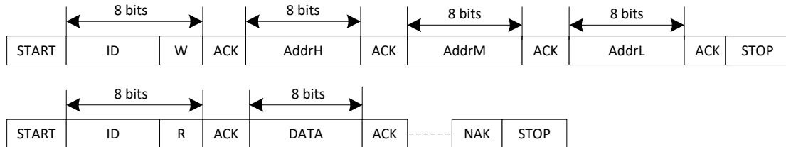
Figure 7- 5 Read format in DMA mode
